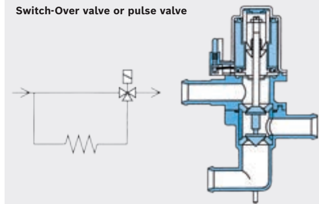
Switch-Over valve or pulse valve
